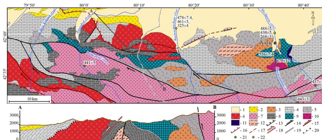
Fig. 3. Geological map of the watershed Ulken Kokpak – Muzhaerte.
