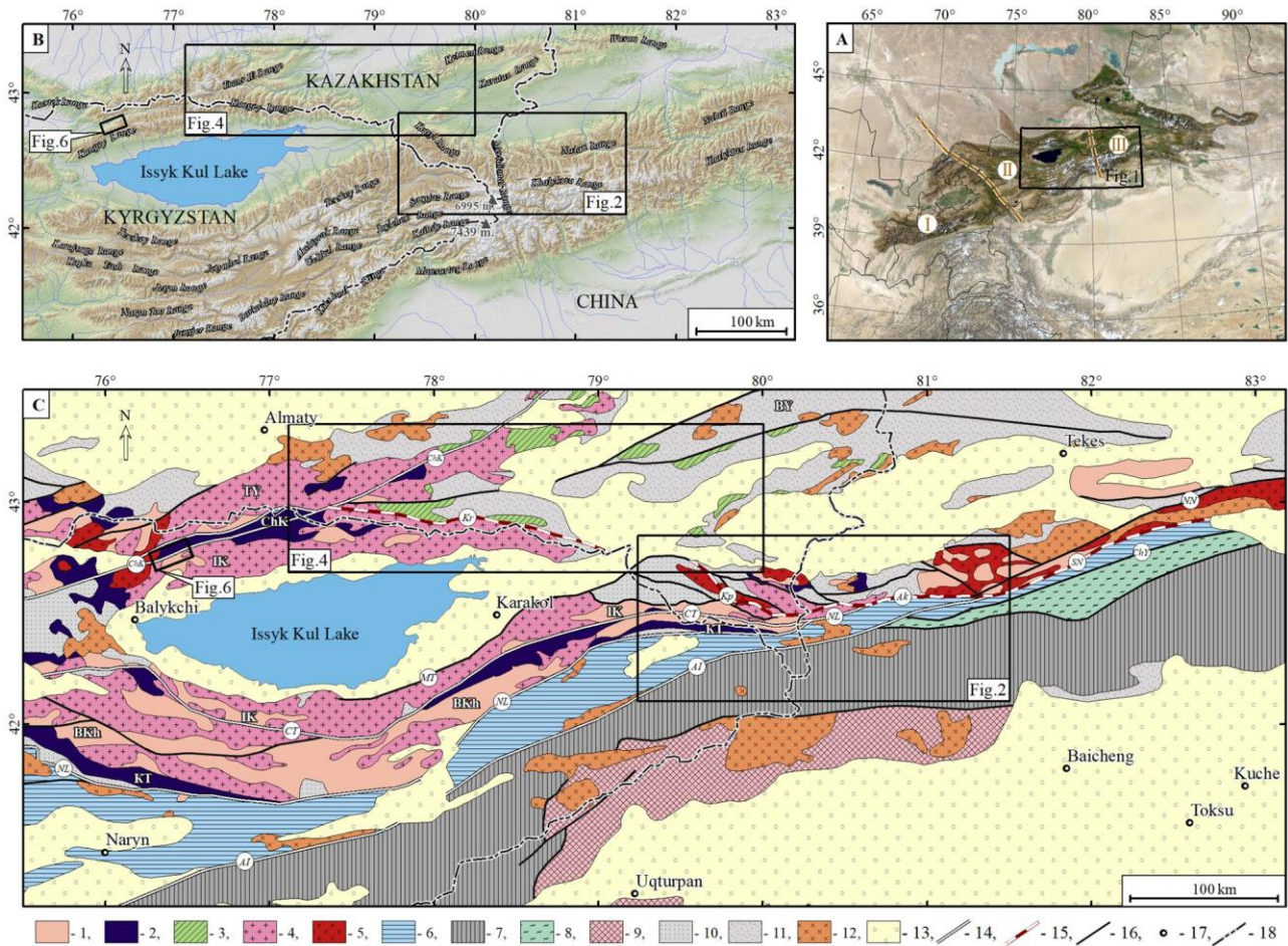
Fig. 1. Orographic scheme (1A,B) and Tectonic map of the Paleozoic formations of Central and Eastern Tianshan (1C), modified after (Alexeiev et al., 2019; Mikolaichuk et al., 2020; “XBGMR,” 1975–1981). Inset 1A shows the scheme of the geographic provinces after (Burtman, 2006), Tianshan: I – Western, II – Central, III – Eastern.
