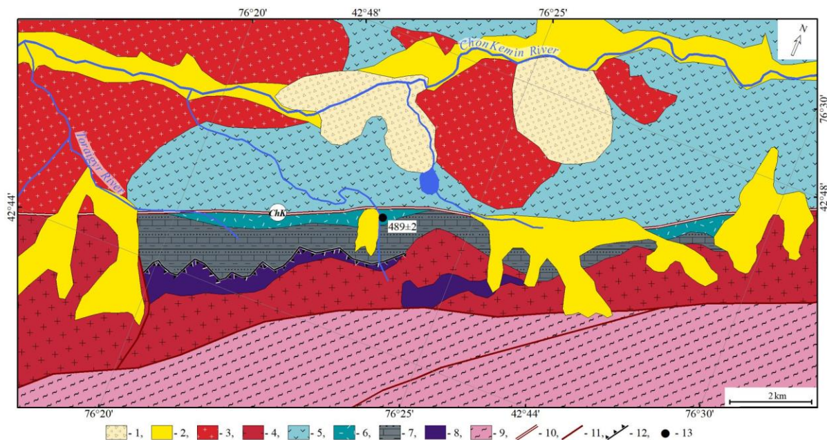
Fig. 6. Lower Paleozoic units of the Issyk-Kul terrane on the left side of the Chon Kemin River.
