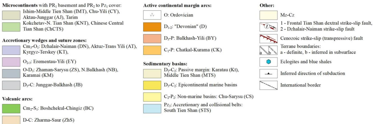
Fig. 8. Tectonic scheme of Paleozoic units in Southern Kazakhstan and Tianshan, modified after (Windley et al., 2007; Kröner et al., 2011a).
